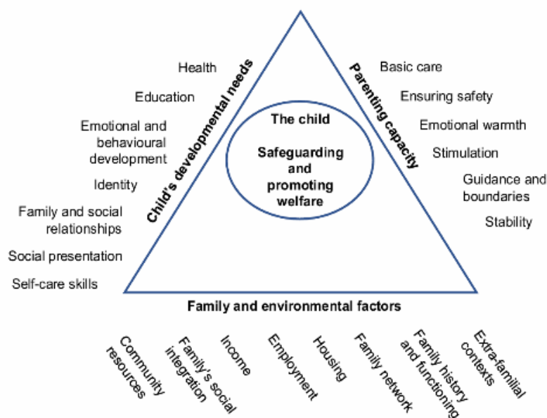
Figure 1: Assessment framework
